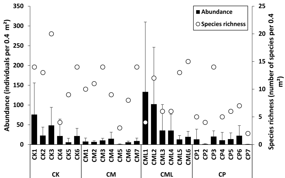
Figure 3. Mean Mollusca abundance ( \bar{x} ) (with standard deviation) and total species richness ( \mu ) per 0.4 m 2 at the 26 stations of the four channels sampled four times from spring 2016 to winter 2017. CP: Ben Khlaf; CML: Maltine; CK: Kneiss; CM: Mimoun.
