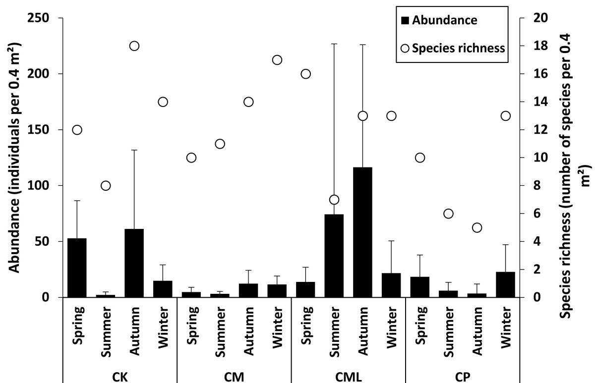
Figure 5. Mean Mollusca abundance ( \nu ) (with standard deviation) and total species richness ( \mu ) per 0.4 \text{ m}^2 in the four channels sampled during the four sampling seasons from spring 2016 to winter 2017. CP: Ben Khlaf; CML: Maltine; CK: Kneiss; CM: Mimoun.
