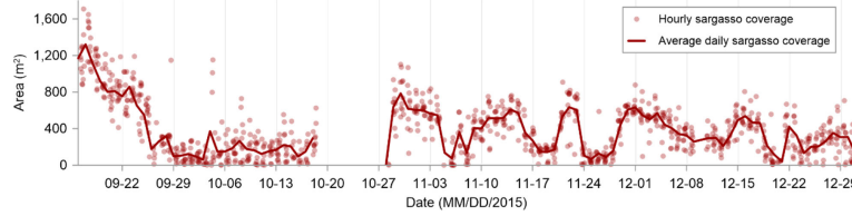
FIGURE 9 Time series of the coverage of beach-cast vegetation (mostly sargasso) for the beach section studied, at Puerto Morelos, September–December, 2015. There are no data in mid-October due to camera failure.
