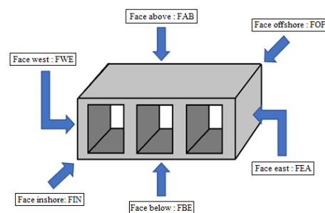
Figure 3. Designations of the six faces of the experimental blocks.
