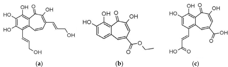
Figure 1. (a) Examples of natural benzotropolones Fomentariol; (b) Goupilone A; (c) Crocipodin.
