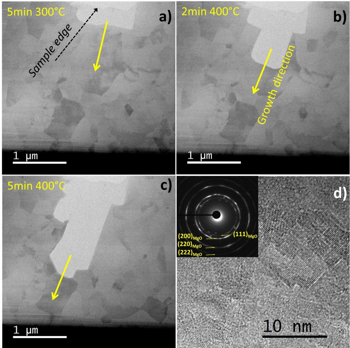
Figure2: STEM-BF images showing the growth of MgO inside the UFG Mg at low partial pressure of \text{O}_2 and \text{H}_2 (below 10^{-5} Pa) (a) after 5min at 300°C, (b) after 2min at 400°C and (c) after 5min at 400°C. (d) HRTEM image taken in the oxidized region showing the nanoscaled structure of the MgO oxide, confirmed by the SAED (inset)
