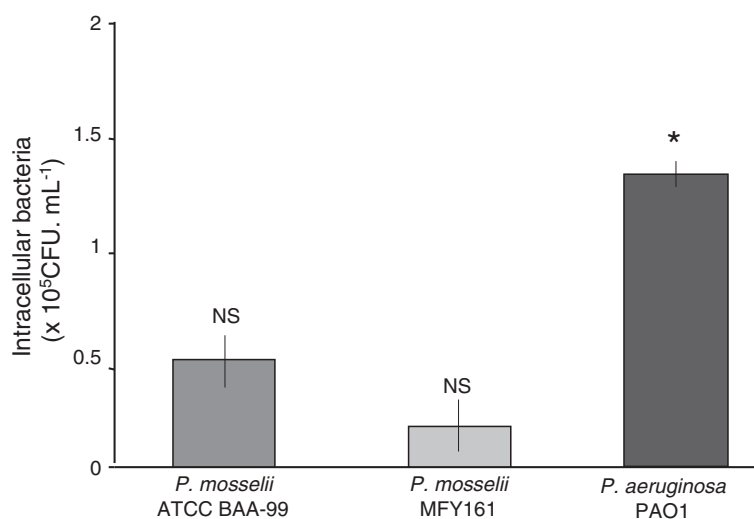
Figure 2 Invasive capacity of P. mosselii ATCC BAA-99, P. mosselii MFY161 and P. aeruginosa PAO1. 4 h after infection of Caco-2/TC7 cells with the bacteria, extracellular germs were killed by gentamicin. Cells were lysed and the intracellular bacteria were enumerated by plating onto nutrient agar medium. Results were calculated as the mean values (+/-SEM) of three independent experiments. * P < 0.05 versus P. mosselii ATCC BAA-99 and P. mosselii MFY161, NS not significant between P. mosselii ATCC BAA-99 and P. mosselii MFY161.
