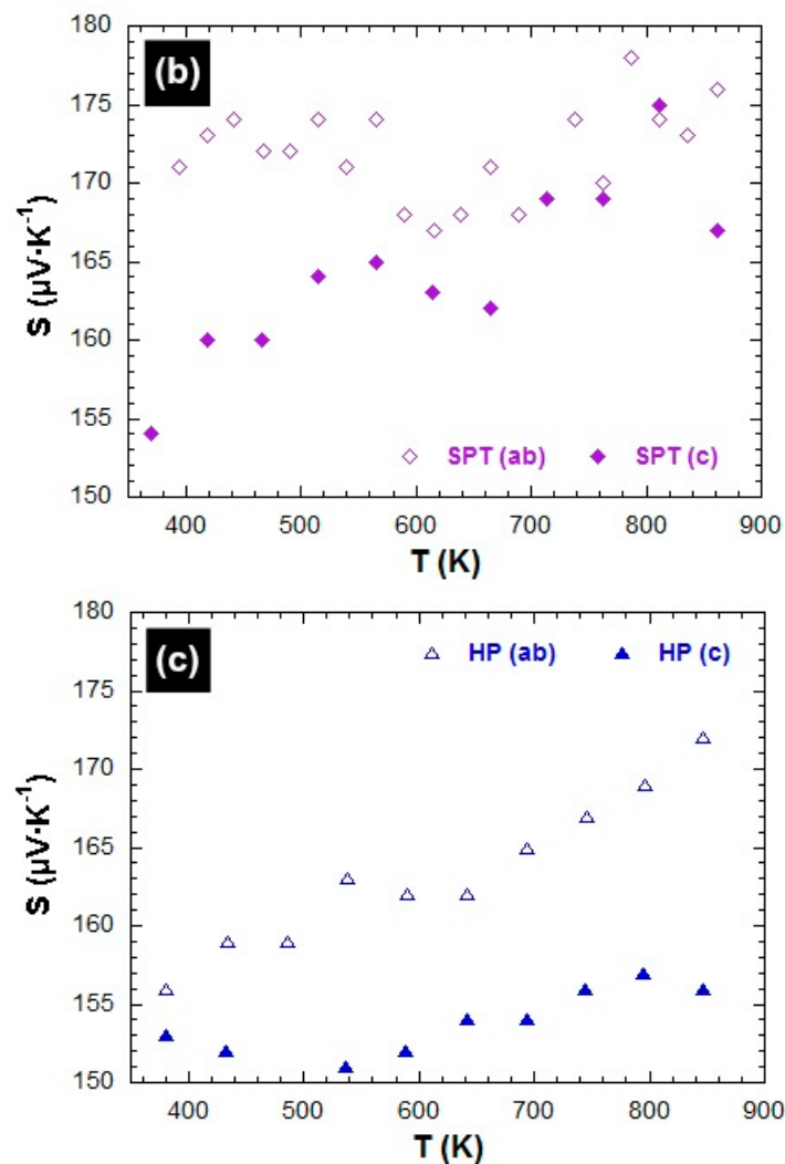
Figure 6. Temperature dependence of the Seebeck coefficient measured parallel ( S^{\text{c}} ) and perpendicular ( S^{\text{ab}} ) to the mean c^* -axis (a) SPS, (b) SPT, and (c) HP stacks.
