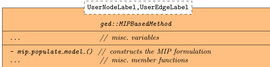
Fig. 6. The interface ged::MIPBasedMethod for methods based on MIP.
