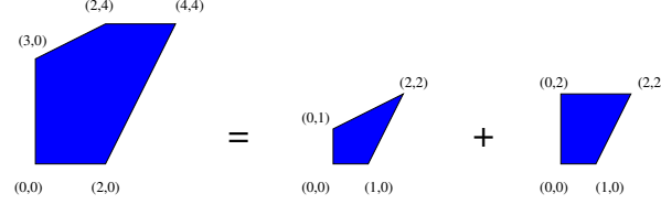
FIGURE 5. The Newton polytopes of the factors q_1 and q_2 of f . We have equality N_f = N_{q_1} + N_{q_2} by a theorem of Ostrowski [22].
