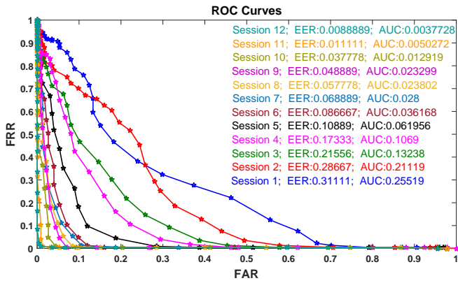
Fig. 1: Illustration of ROC curves and the associated EER and AUC performances of each adaptation session for WEBGREYC database.
