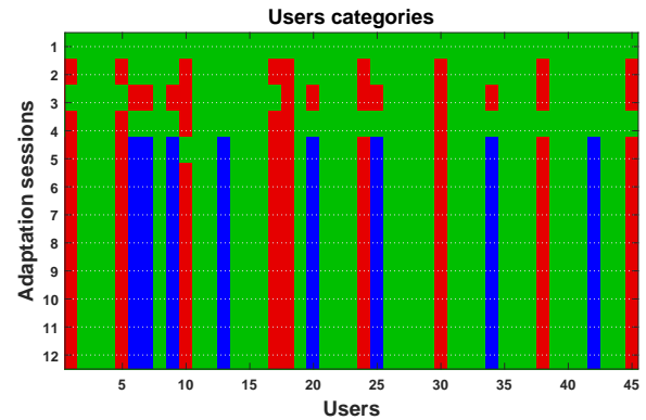
Fig. 5: Distribution of users categories during all adaptation session for WEBGREYC database. The green color illustrates the sheeps class, the red color illustrates the goats class and the blue color illustrates the lambs class.
