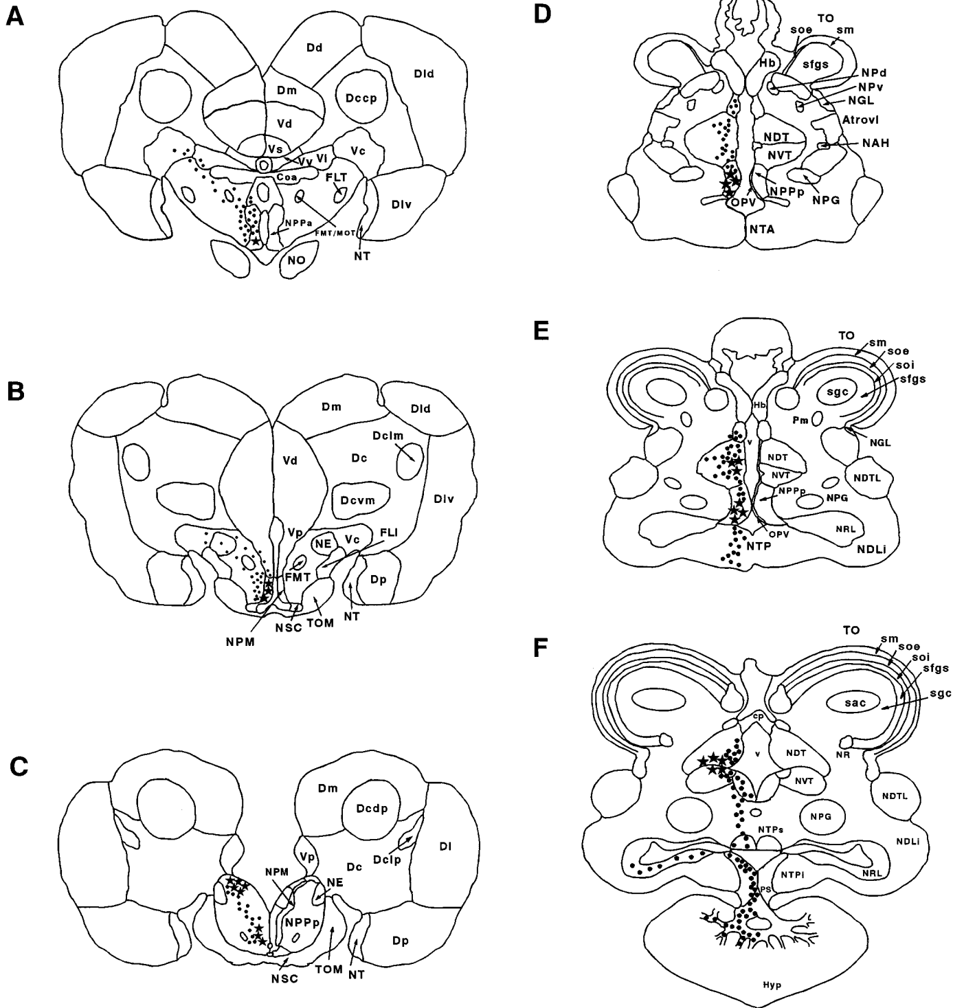
FIG. 2. Schematic frontal sections through the eel brain depicting the distribution of PACAP-immunoreactive cell bodies ( stars ) and fibers ( dots ). The localization of anatomical structures is indicated on the right hemisection. The capital letters (A-I) refer to the rostrocaudal levels of the sections as indicated in Fig. 1. For abbreviations, see Table 2. Figures are taken from the atlas of Medina et al. (39).
